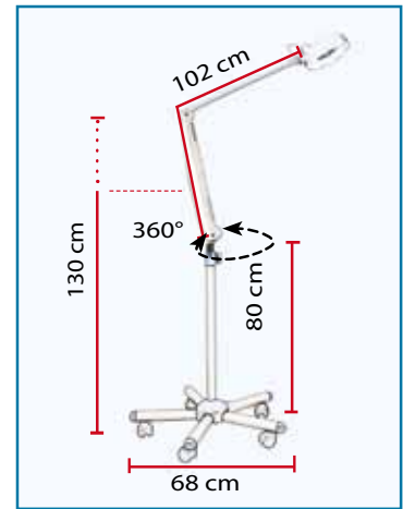
Adjustable height trolley code CH/CIR/R/105
